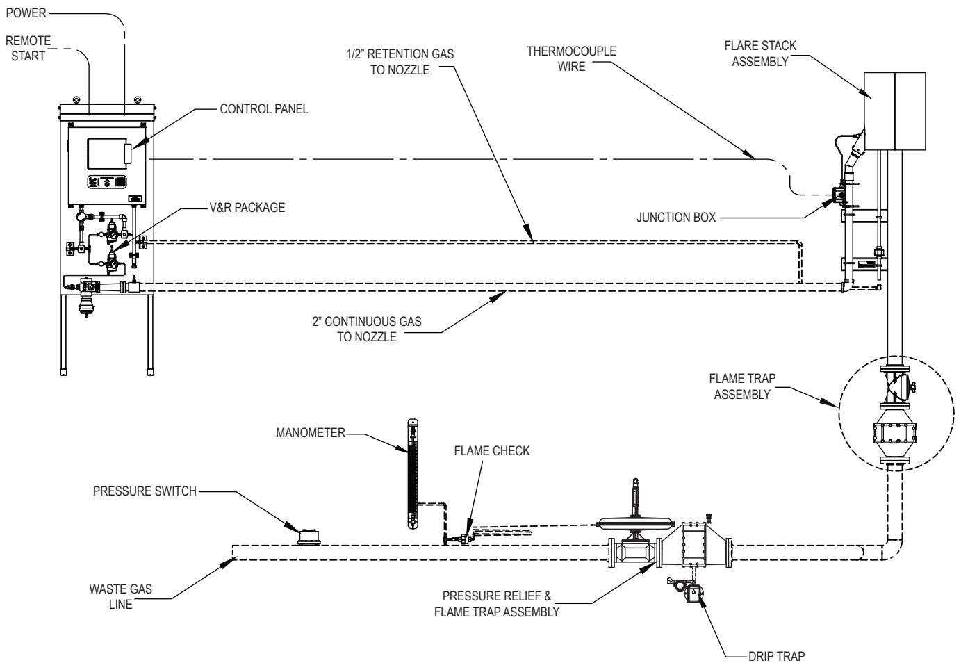
Figure 01: 244W - Typical Installation
